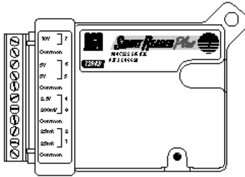
Figure 7-1: SmartReader Plus 7
