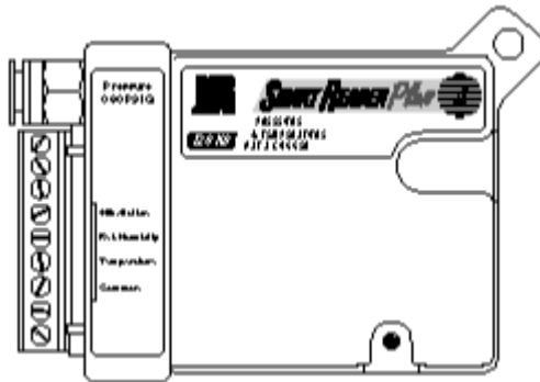
Figure 4-1: SmartReader Plus 4
